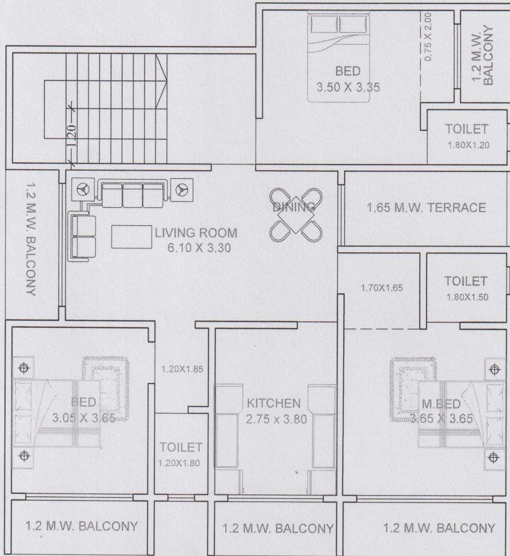
FIRST AND SECOND FLOOR PLAN P LINE - 131.01 SQ M
