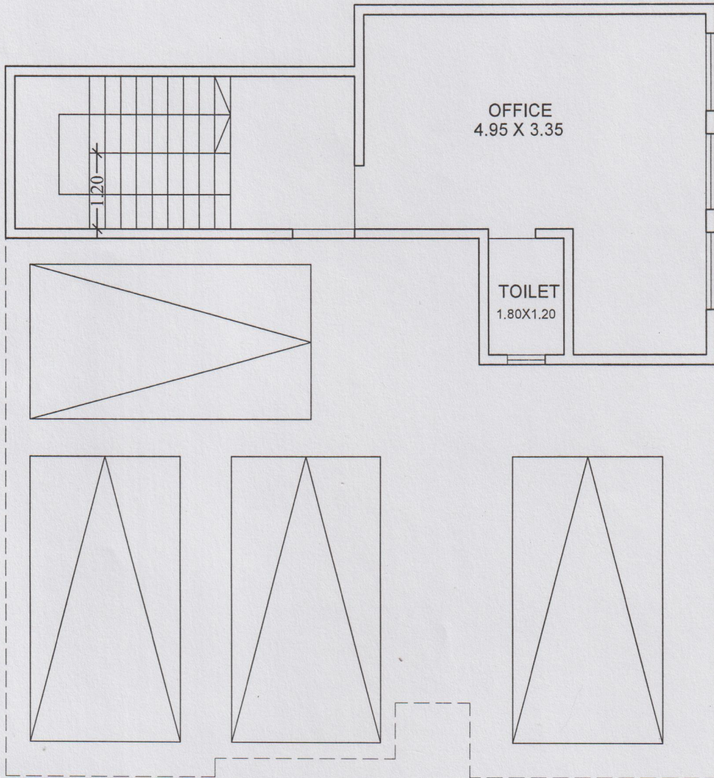
GROUND FLOOR PLAN P LINE - 43.66 SQ M
