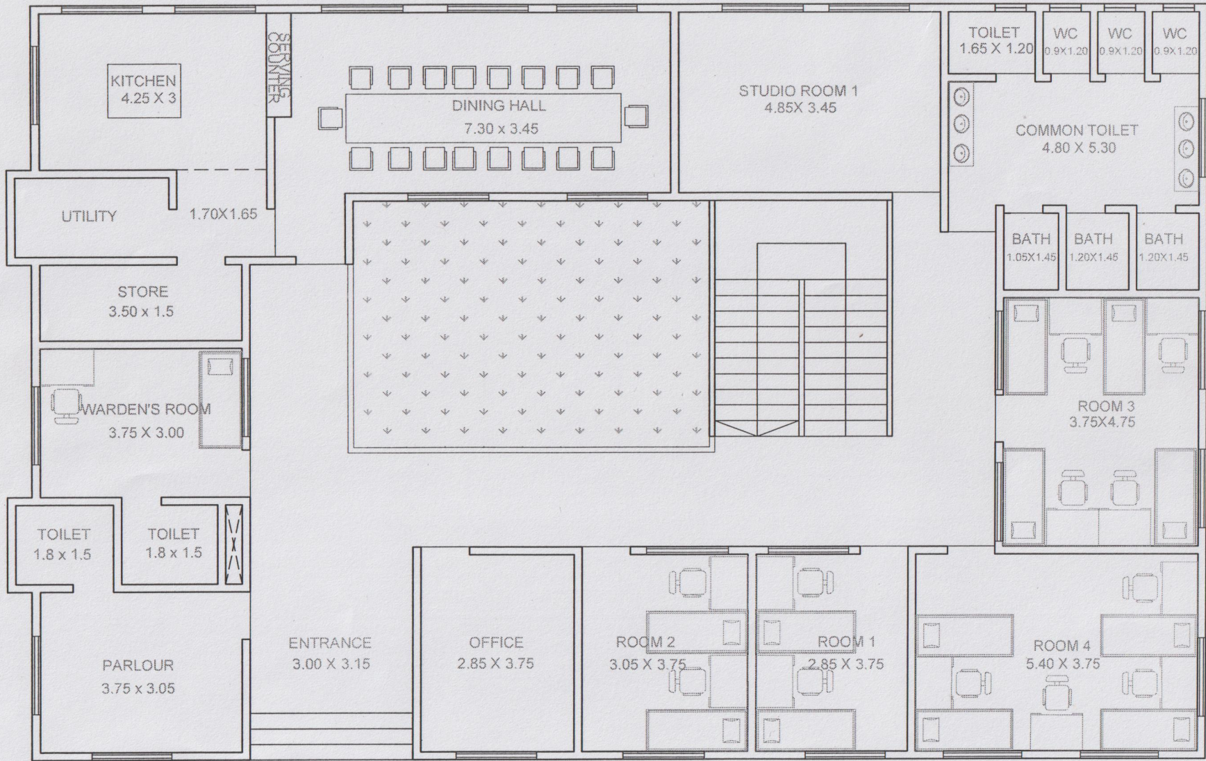
GROUND FLOOR PLAN 286.68 SQ M
